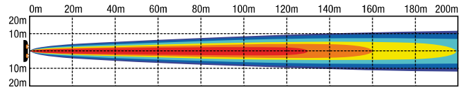
RWL590S Work Lamp Heavy Duty LED 10-30V 90W Square Spot Beam
