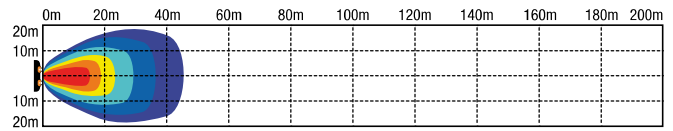
RWL530F Work Lamp Heavy Duty LED 10-30V 30W Square Flood Beam
