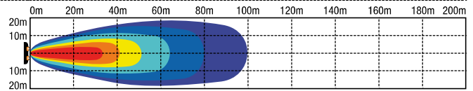
RWL590F Work Lamp Heavy Duty LED 10-30V 90W Square Flood Beam
